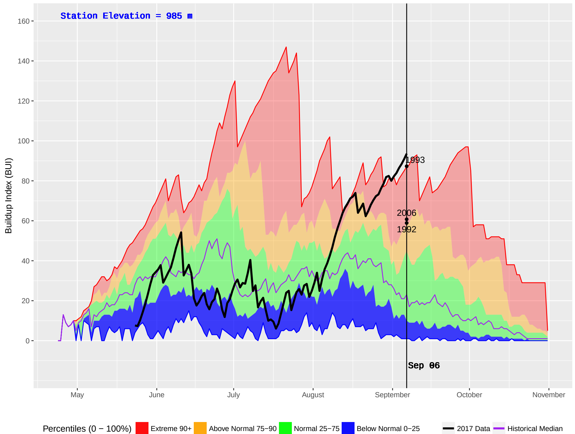
SIFTON (152) : Historical (1988–2016) and Current (2017) Noon Buildup Index (BUI)
