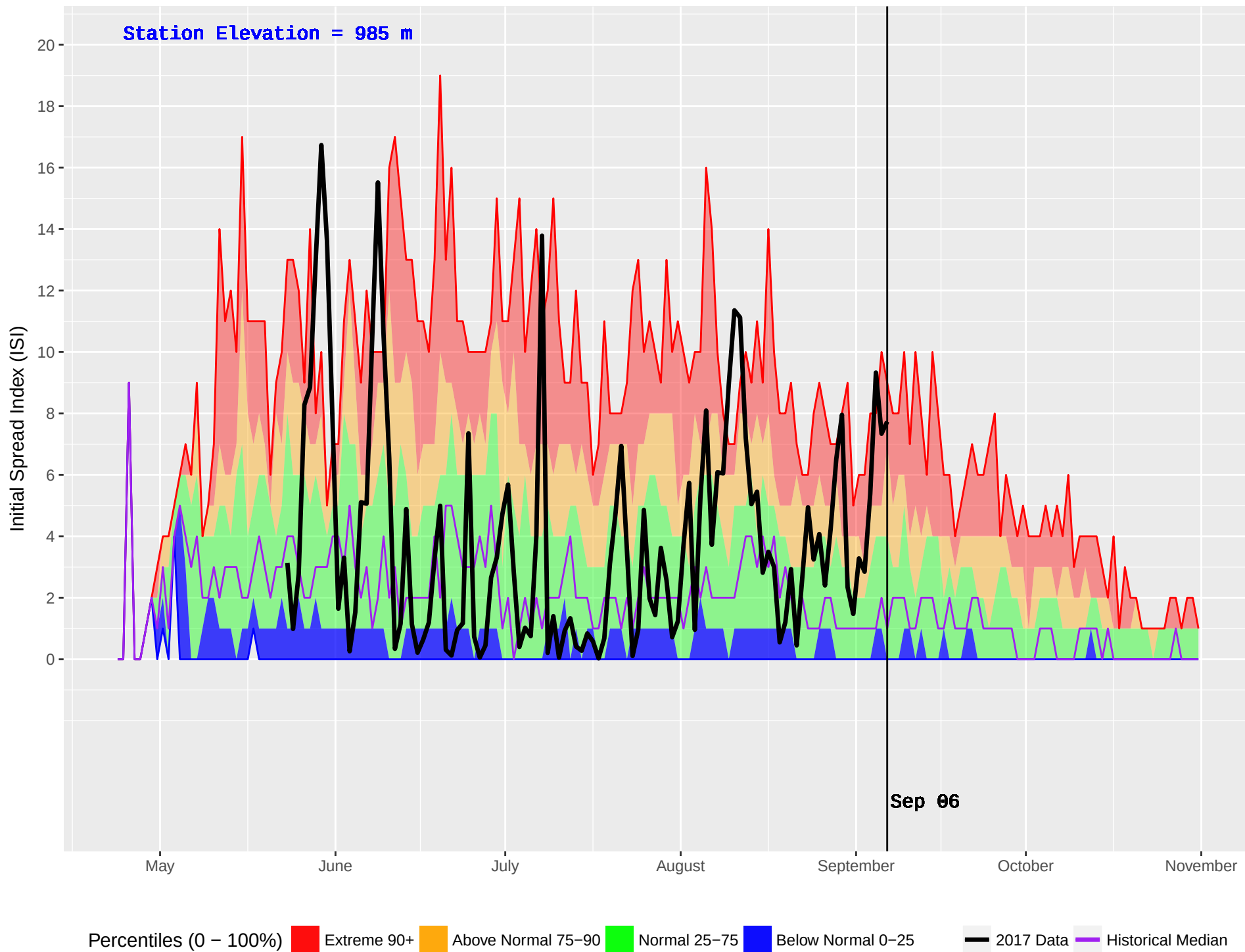
SIFTON (152) : Historical (1988–2016) and Current (2017) Noon Initial Spread Index (ISI)
