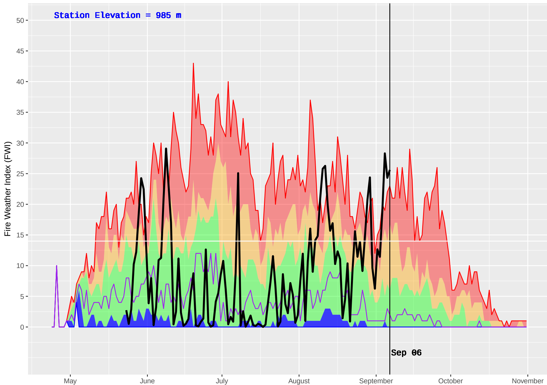
SIFTON (152) : Historical (1988–2016) and Current (2017) Noon Fire Weather Index (FWI)
