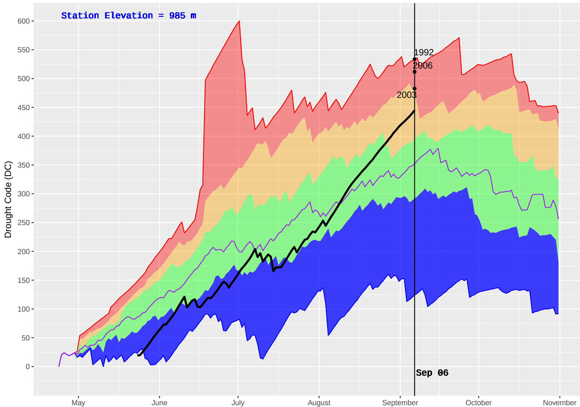
SIFTON (152) : Historical (1988–2016) and Current (2017) Noon Drought Code (DC)
