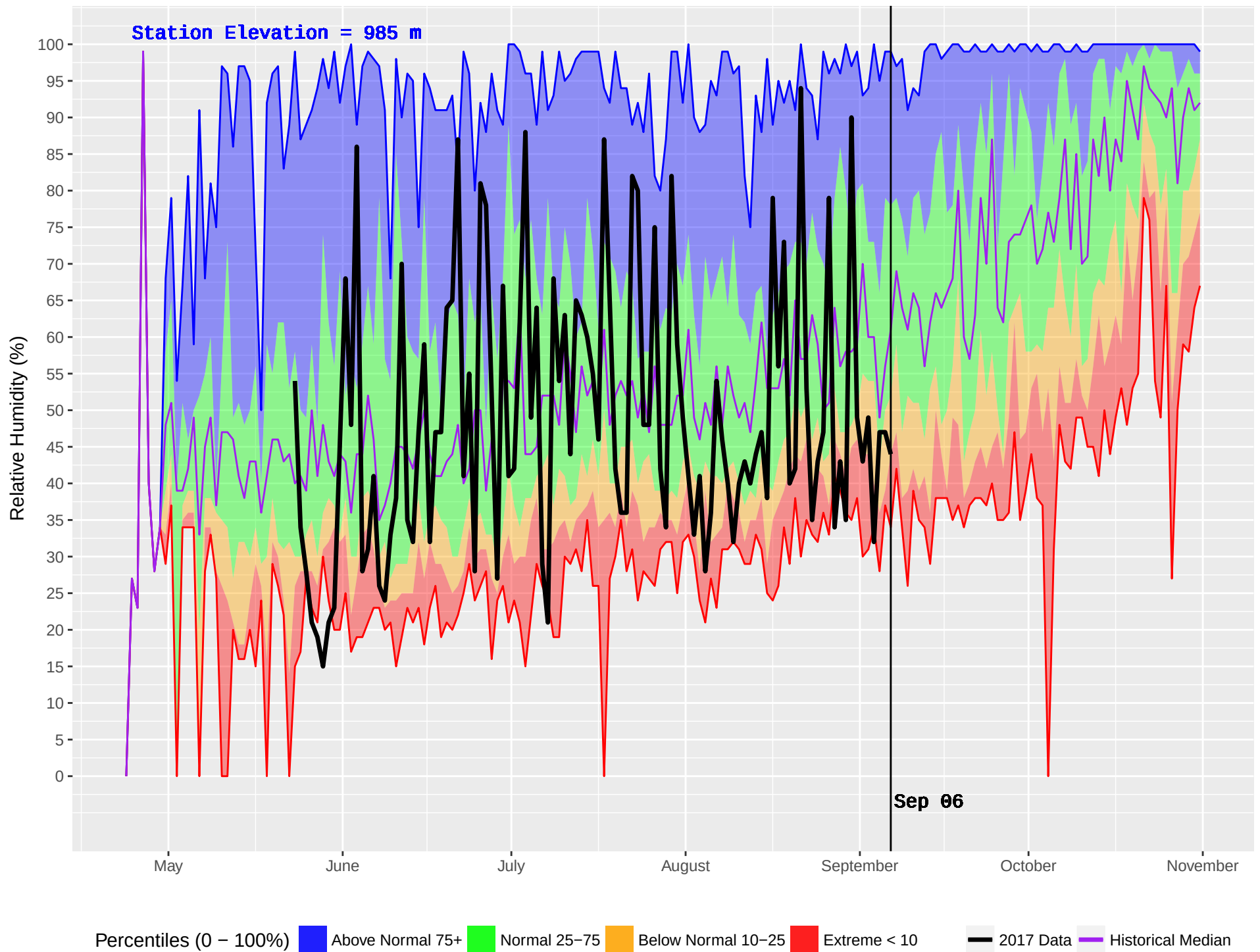
SIFTON (152) : Historical (1988–2016) and Current (2017) Noon Relative Humidity
